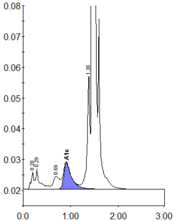
Peak table - ID: 10367163
